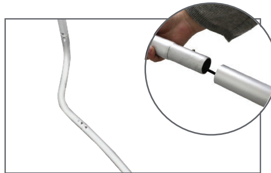
Step 2: Assemble the frame starting with the curved 90° degree poles by matching the corresponding numbers located on each pole. Repeat for the remaining poles. The straight poles have elastic connectors for easy assembly.
